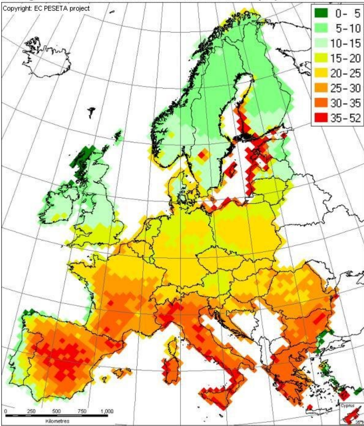
Average annual differences in heat-related deaths / 100,000 people for 2071-2100
