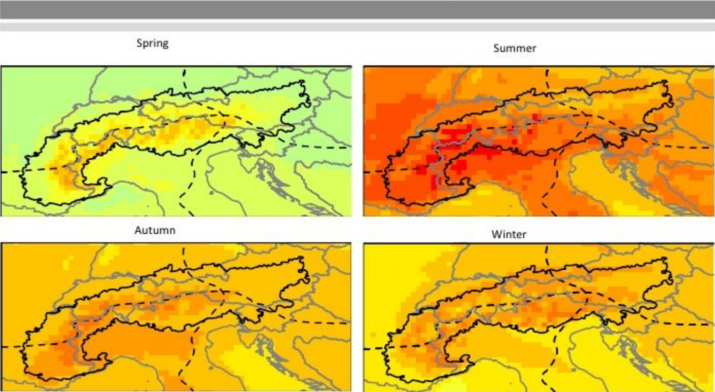
T increase 2071-2100 (CLM A1B)
